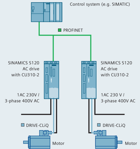
SINAMICS S120 single-axis drive
